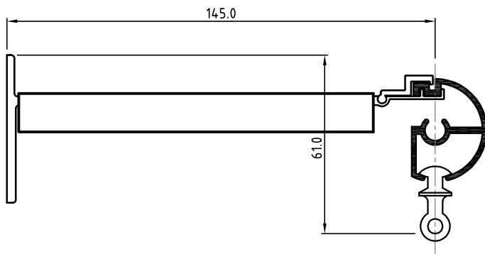
✱ 35mm Premo 145mm Bracket
